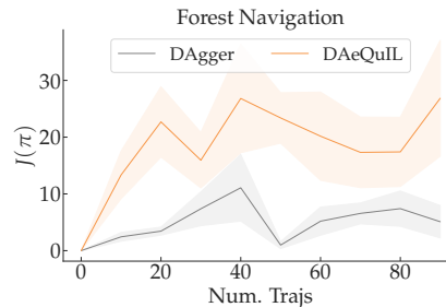
Figure 9. J(\pi) is the longitudinal distance into the forest the learner is able to progress. All experiments are run on the forest layout shown in Fig. 4 and standard errors are computed across 10 trials.
